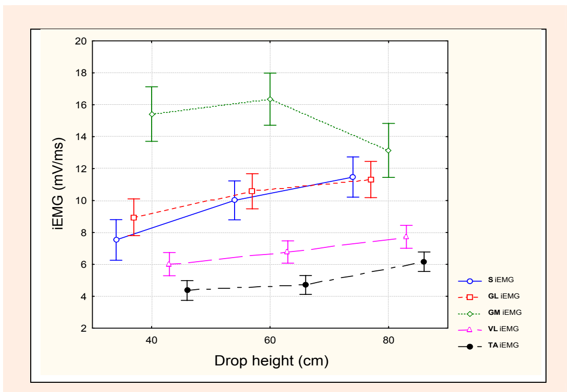
Figure 4. Modulation of integral EMG (iEMG) related to drop height, for all observed muscles (GL, GM, S, VL, TA). Vertical bars denote 0.95 confidence intervals.
