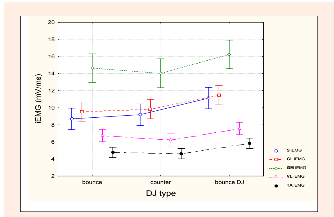
Figure 6. Modulation of integral EMG (iEMG) related to DJ type, for all observed muscles (GL, GM, S, VL, TA). Vertical bars denote 0.95 confidence intervals.
