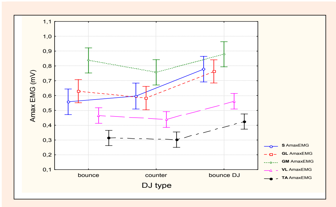
Figure 5. Modulation maximal EMG amplitude (AmaxEMG) related to DJ type, for all observed muscles (GL, GM, S, VL, TA). Vertical bars denote 0.95 confidence intervals.
