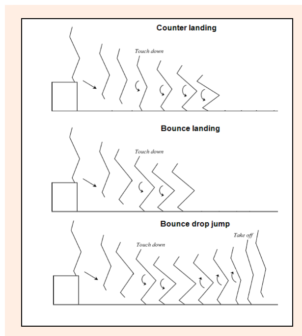
Figure 1. The illustration of proposed three types of deep jump (Modified illustration from Horita et al., 2002).
