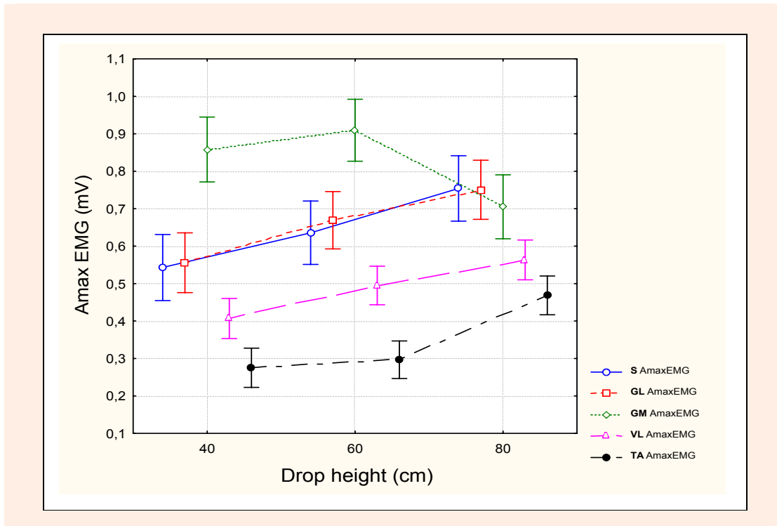
Figure 3. Modulation of maximal EMG amplitude (AmaxEMG) related to drop height, for all observed muscles (GL, GM, S, VL, TA). Vertical bars denote 0.95 confidence intervals.
